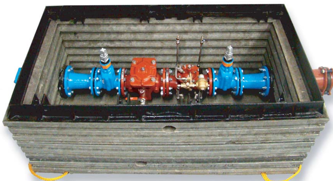
Pressure Reduction Valve Chamber
